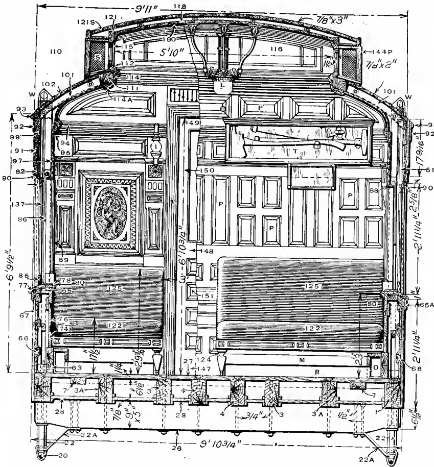
Fig. 540. Transverse Section Showing Interior. FIRST-CLASS PASSENGER COACH.
